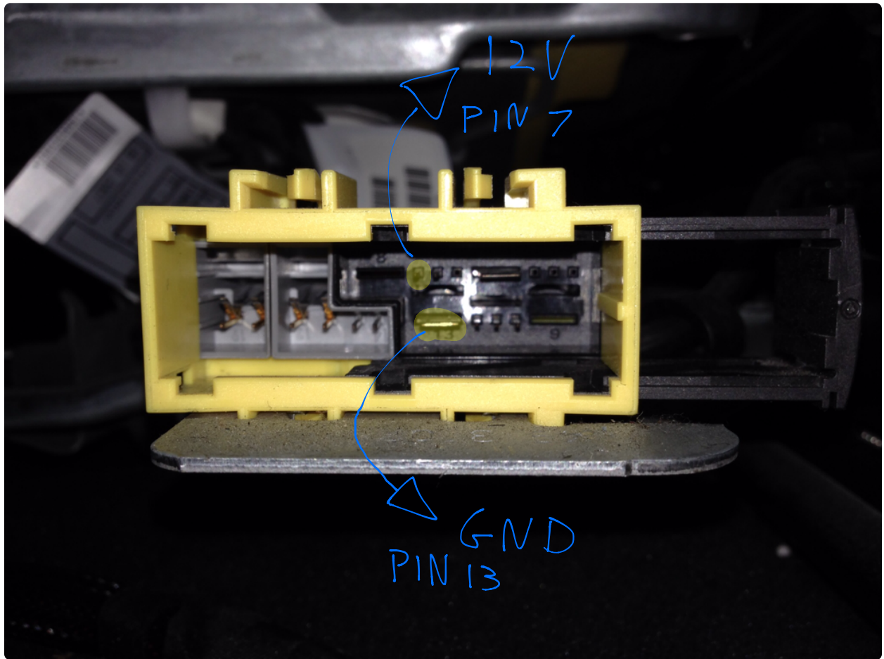
Seat harness
