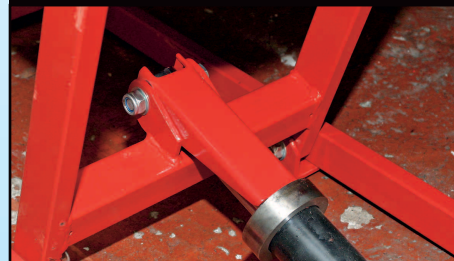
Flip down safety catch, which prevents ram retracting should the hydraulics fail.
